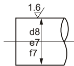
Mating Shaft
